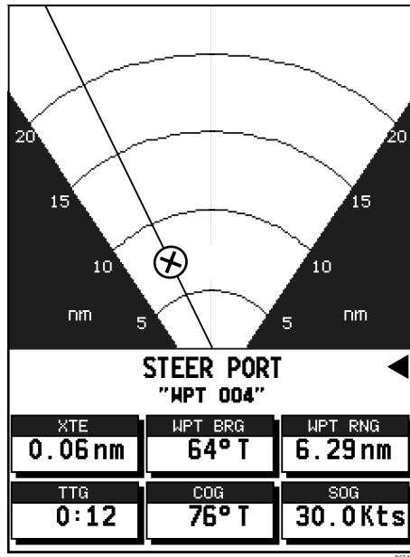
Figure 5-6: BDI Display
